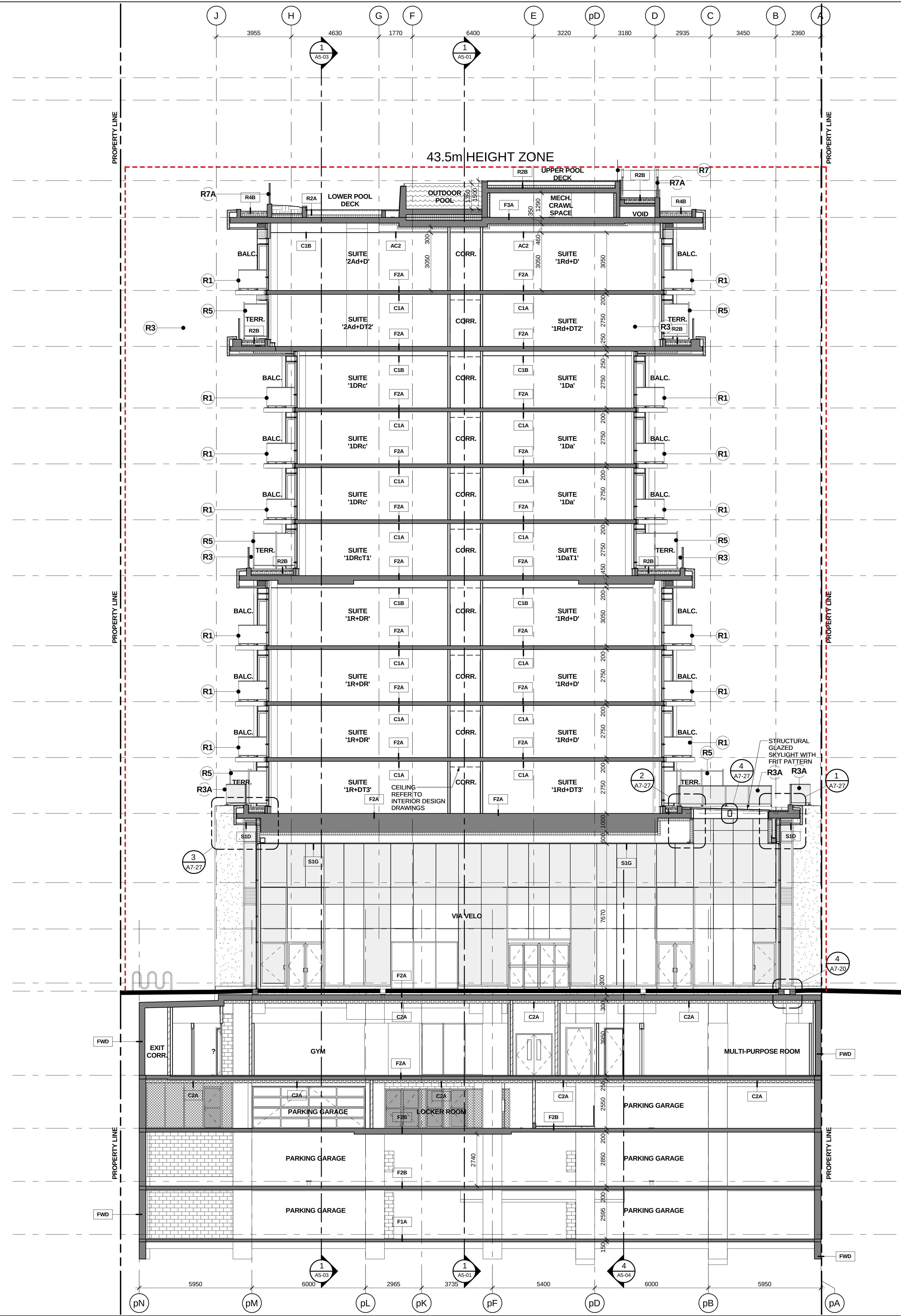
East - West Building Section Along Gridline p8/10 Scale: 1 : 100 A5-02
