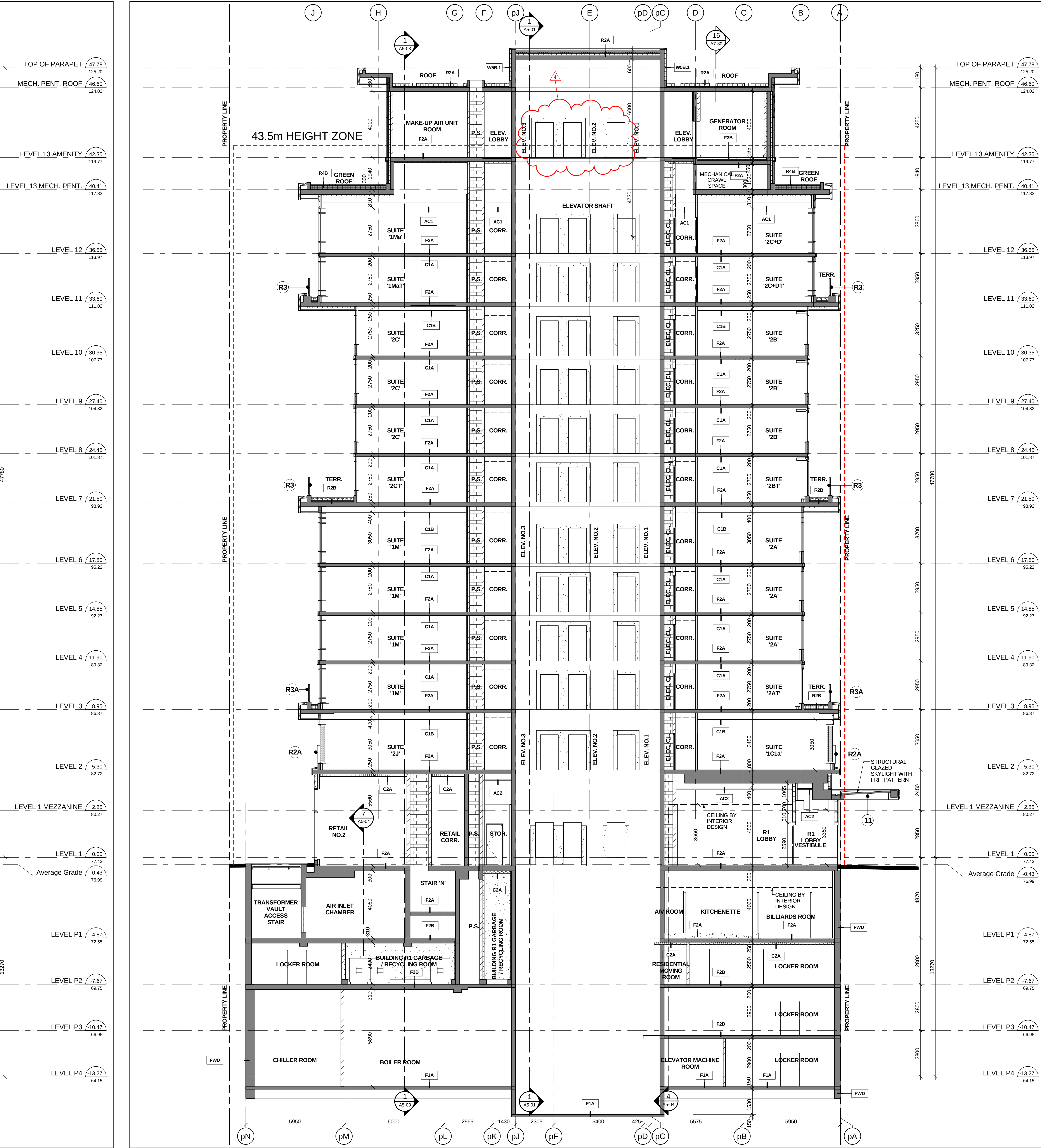
East - West Building Section Along Gridline p8/10 Scale: 1 : 100 A5-02
