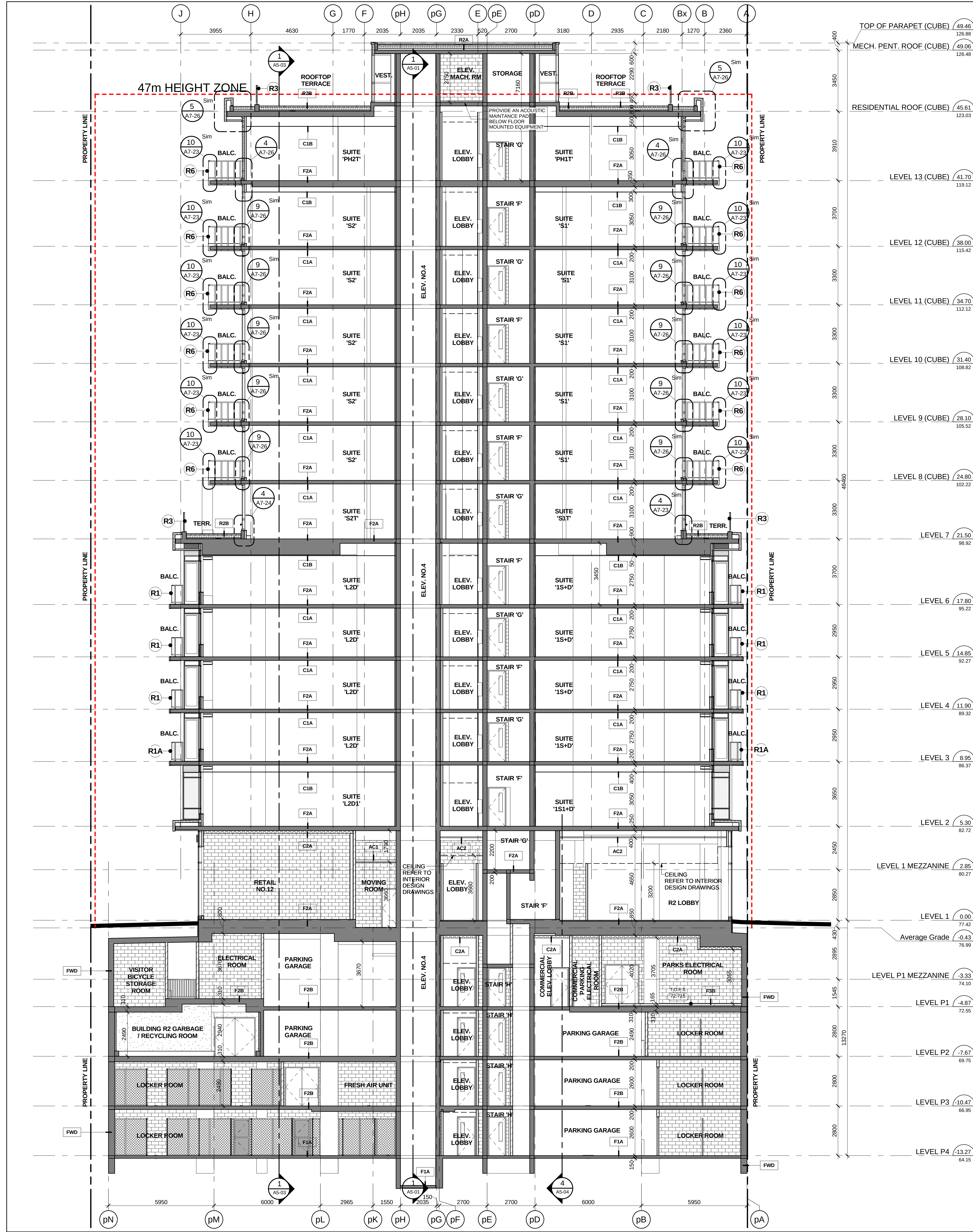
East - West Building Section Along Gridline p22 Scale: 1 : 100 A5-02
